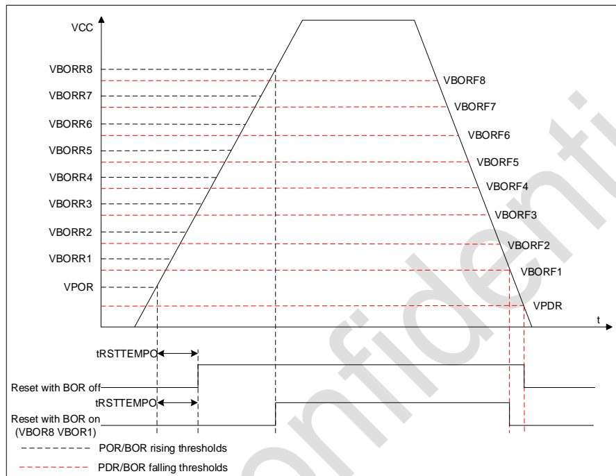
Figure 2-3 POR/PDR/BOR threshold
