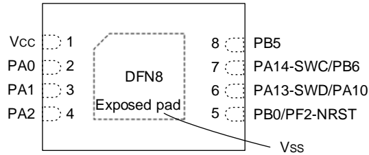
Figure 3-14 DFN8(3*2) PY32F003L2xDx (Top view)
