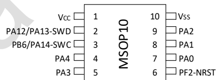
Figure 3-11 MSOP10 PY32F003A1xNx (Top view)
